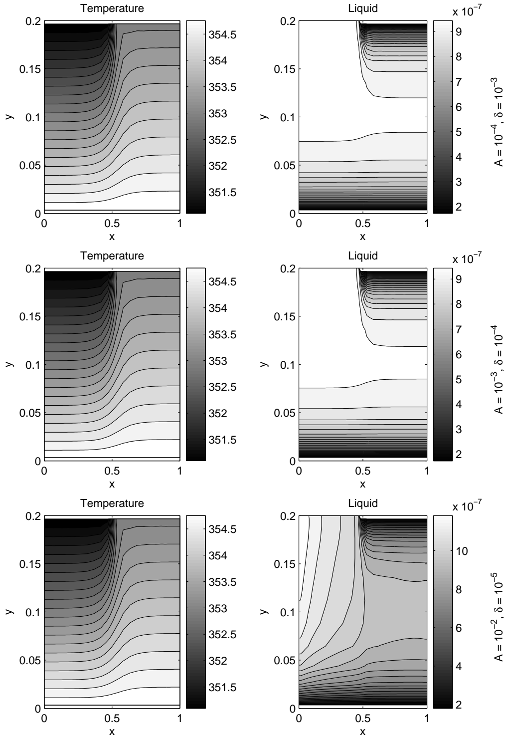
Figure 9.2. Spectral computations of (9.2), the hydrothermal equilibrium in GDL. All quantities used for the calculation are known physical constants or parameters supplied by Gore. The only unknowns are A , p , \delta , and B , which characterize our model hydraulic diffusivity. The first figure is essentially linear since variations in \theta have little impact on D_\theta . As \delta decreases, nonlinear behavior becomes more pronounced to a point where the diffusivity varies by a factor of two depending upon the moisture content in the last calculation ( \delta = 10^{-5} ).
