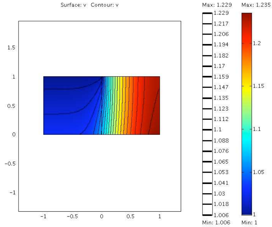
Figure 5.3. Contour plot of water vapor concentration.
