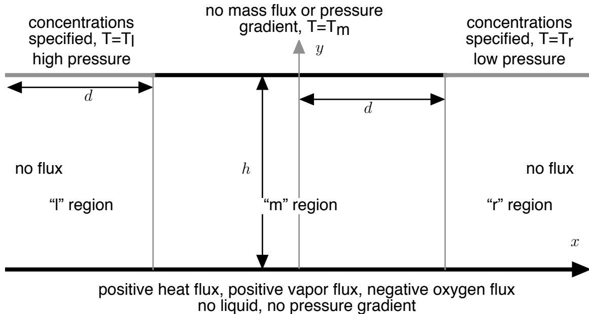
Figure 1.2. This simplified periodic geometry was the focus of our attention during the MPI workshop. The grey lines at the top of the diagram indicate the position of the channel through which the gases flow. We consider only the movement of gas, liquid water, vapor and heat through the rightmost GDM in Figure 1. Note also that the orientation of this diagram has been rotated 90^\circ from Figure 1. (In particular, the cathode to the left of the GDM is now beneath it.)
