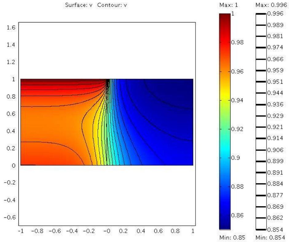
Figure 10.2. Vapor concentration v . Notice the trough near y = 0.5 , -1 < x < 0 .
