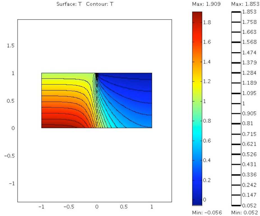
Figure 5.2. Contour plot of temperature.
