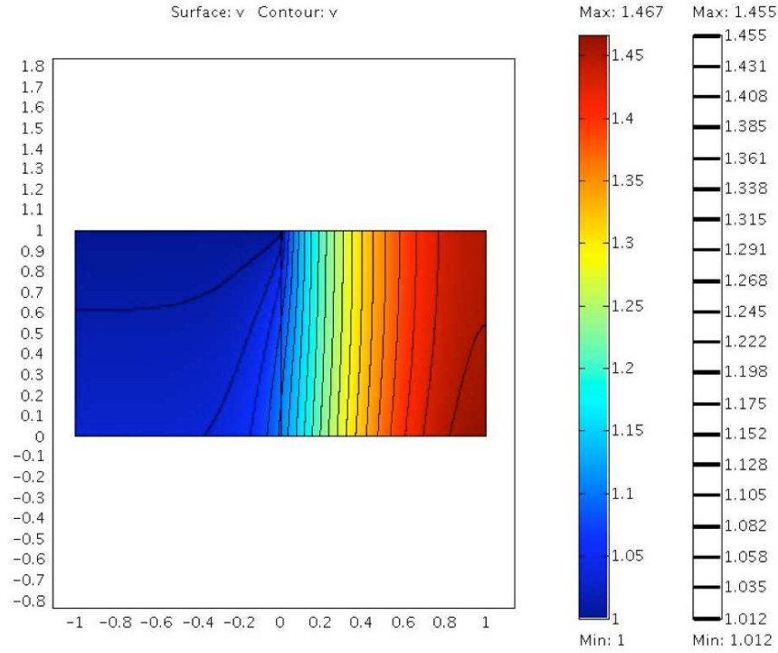
Figure 4.5. Contour plot of water vapor concentration.
