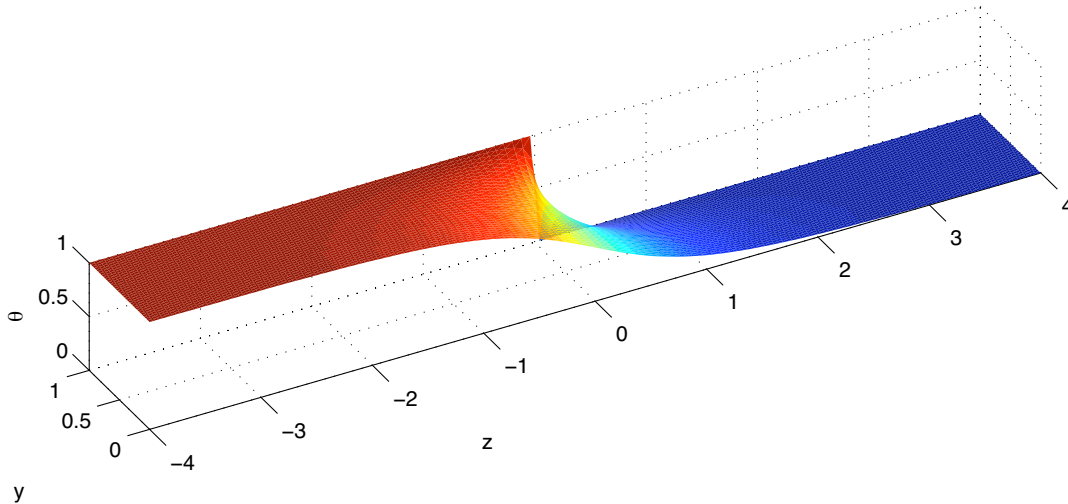
Figure 4.3. 3-D plot of T^i in interior layer.
